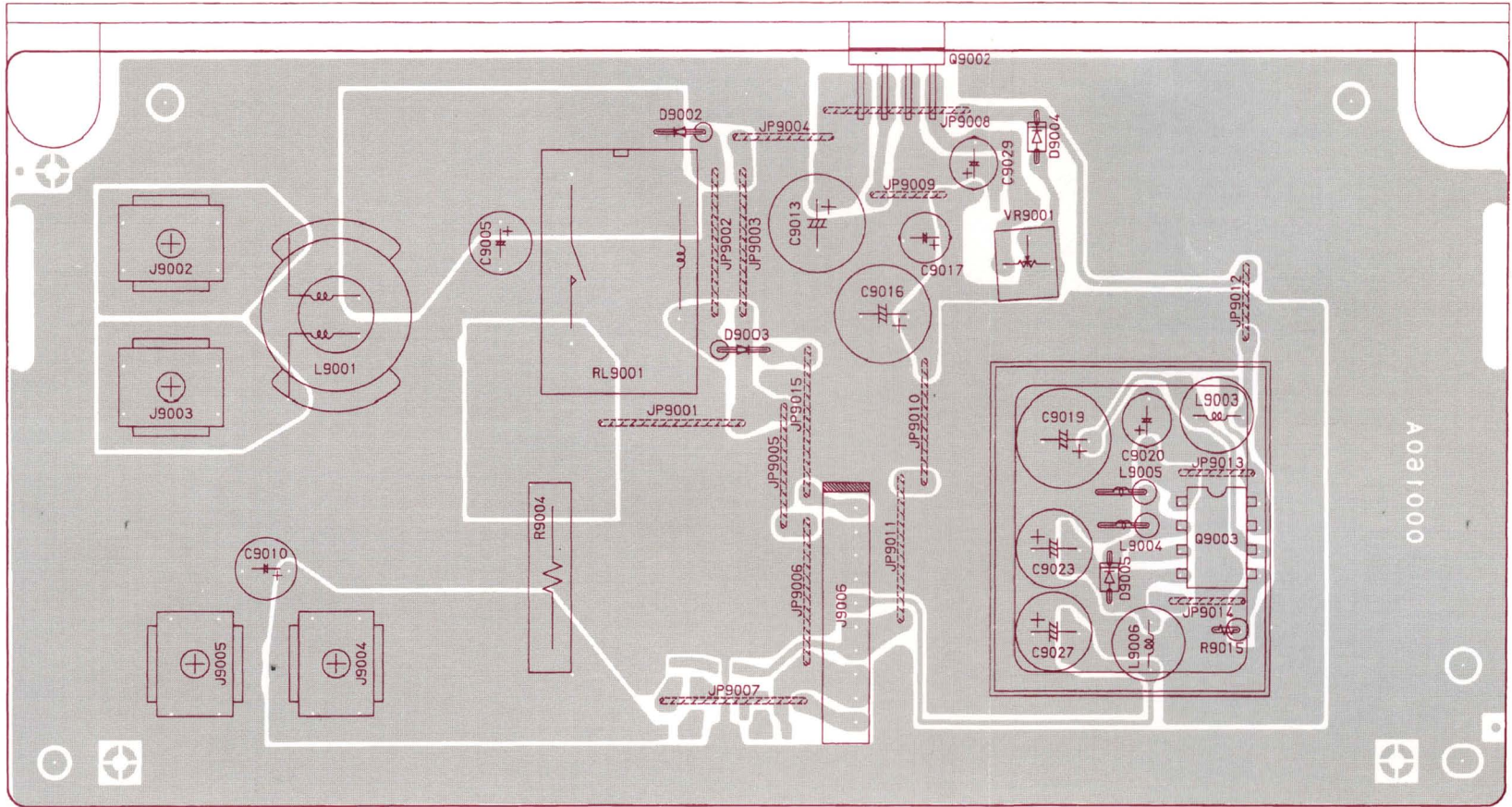
Solder Side
