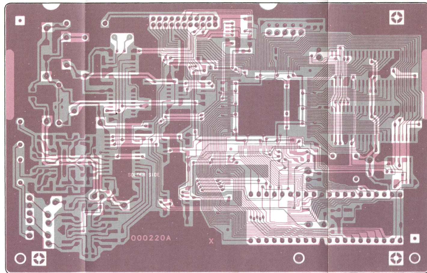
Solder Side
