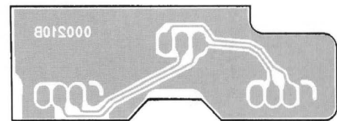
Solder Side
