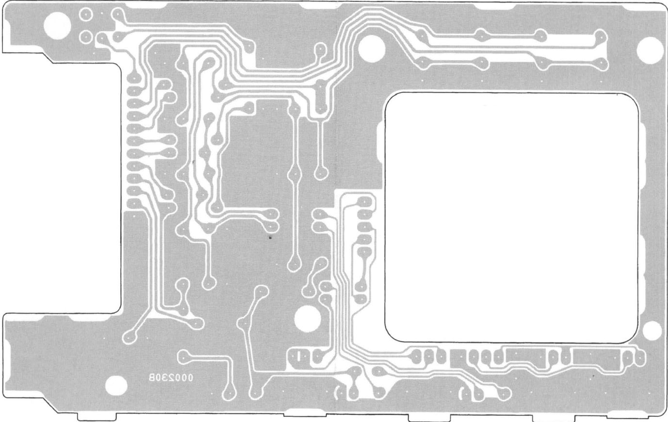
Solder Side
