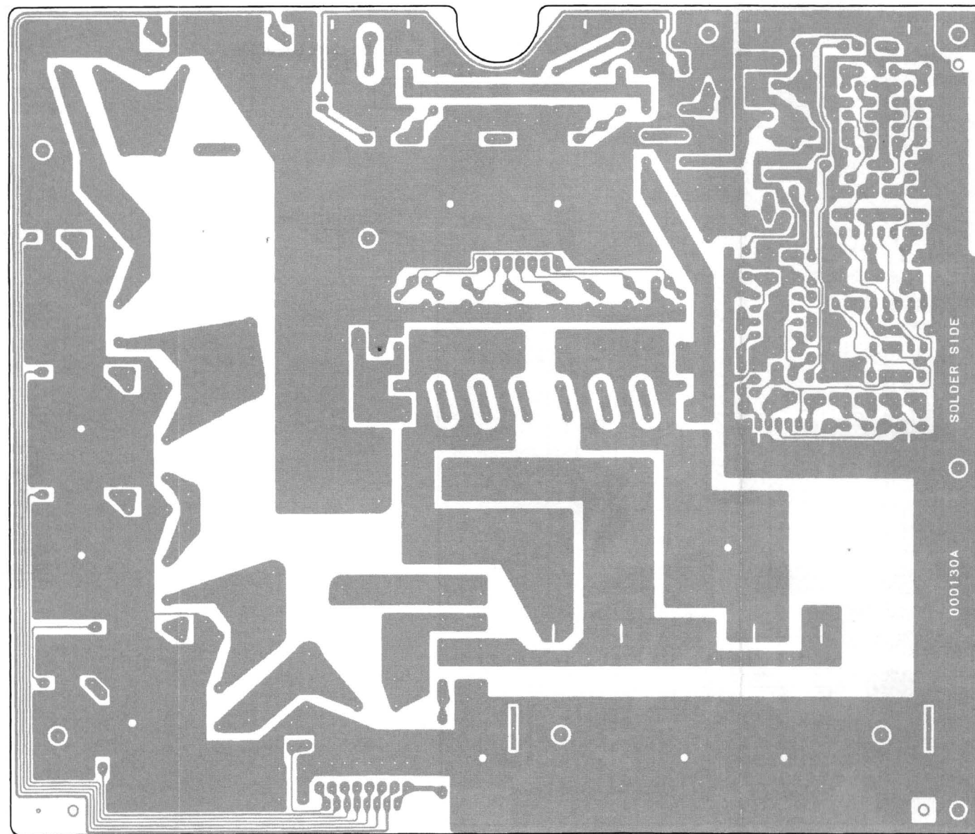
Solder Side
