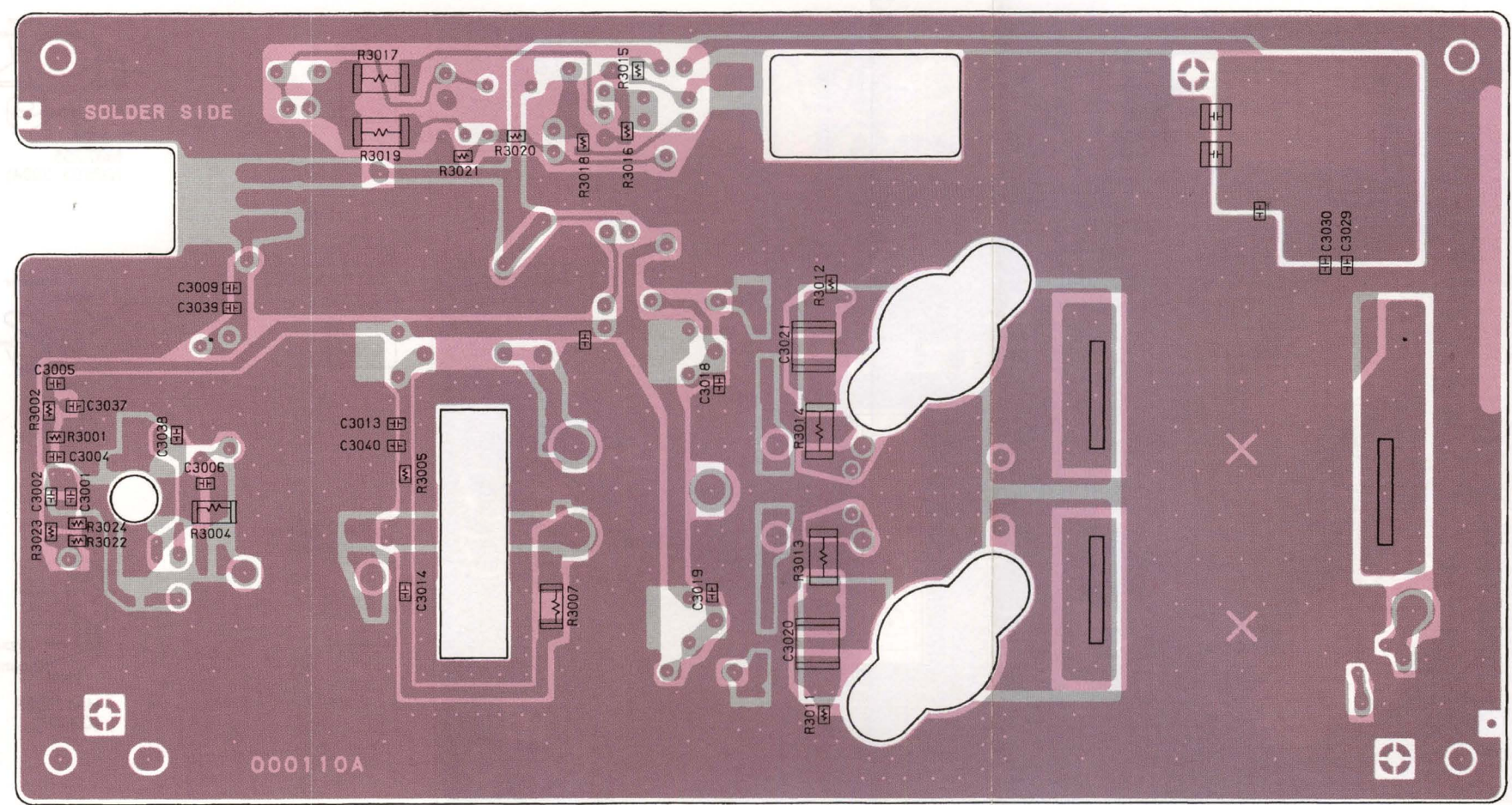
Chip Side
