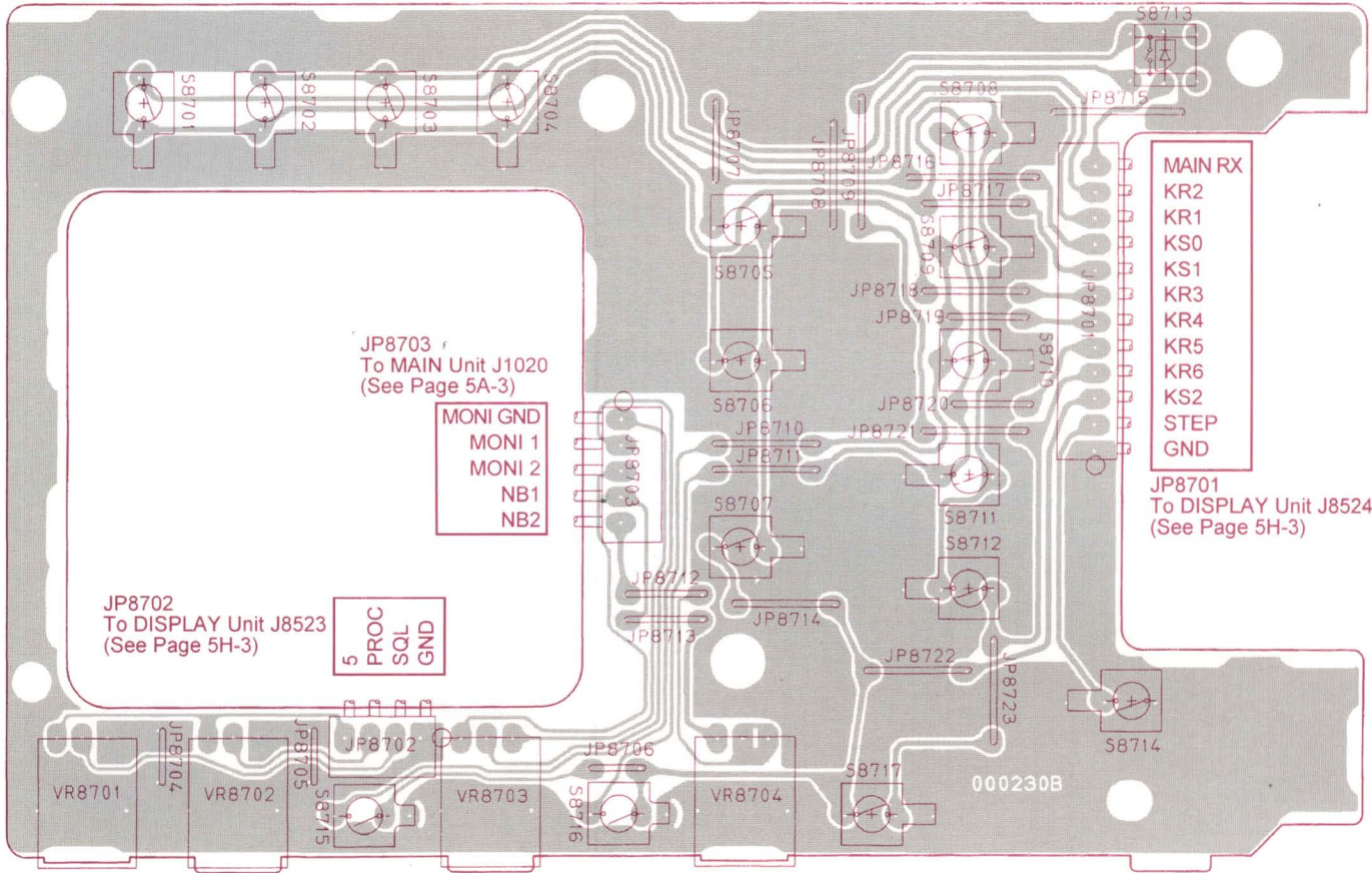
Component Side
