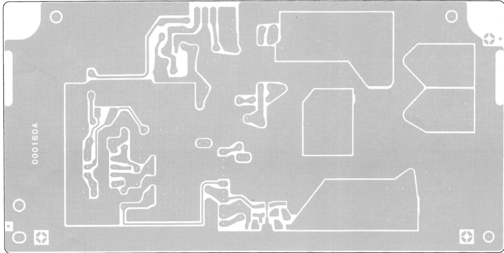
Component Side
