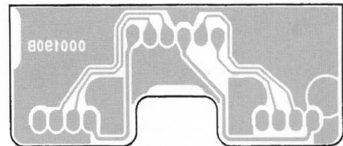
Solder Side
